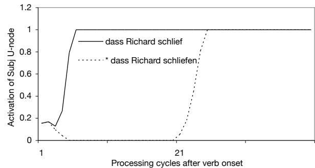
Figure 3. Delayed unification due to missing subject-verb agreement.
