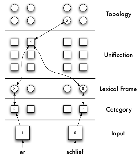
Figure 2. Activation spreading through the SINUS network. The Linear Order layer is not shown.
